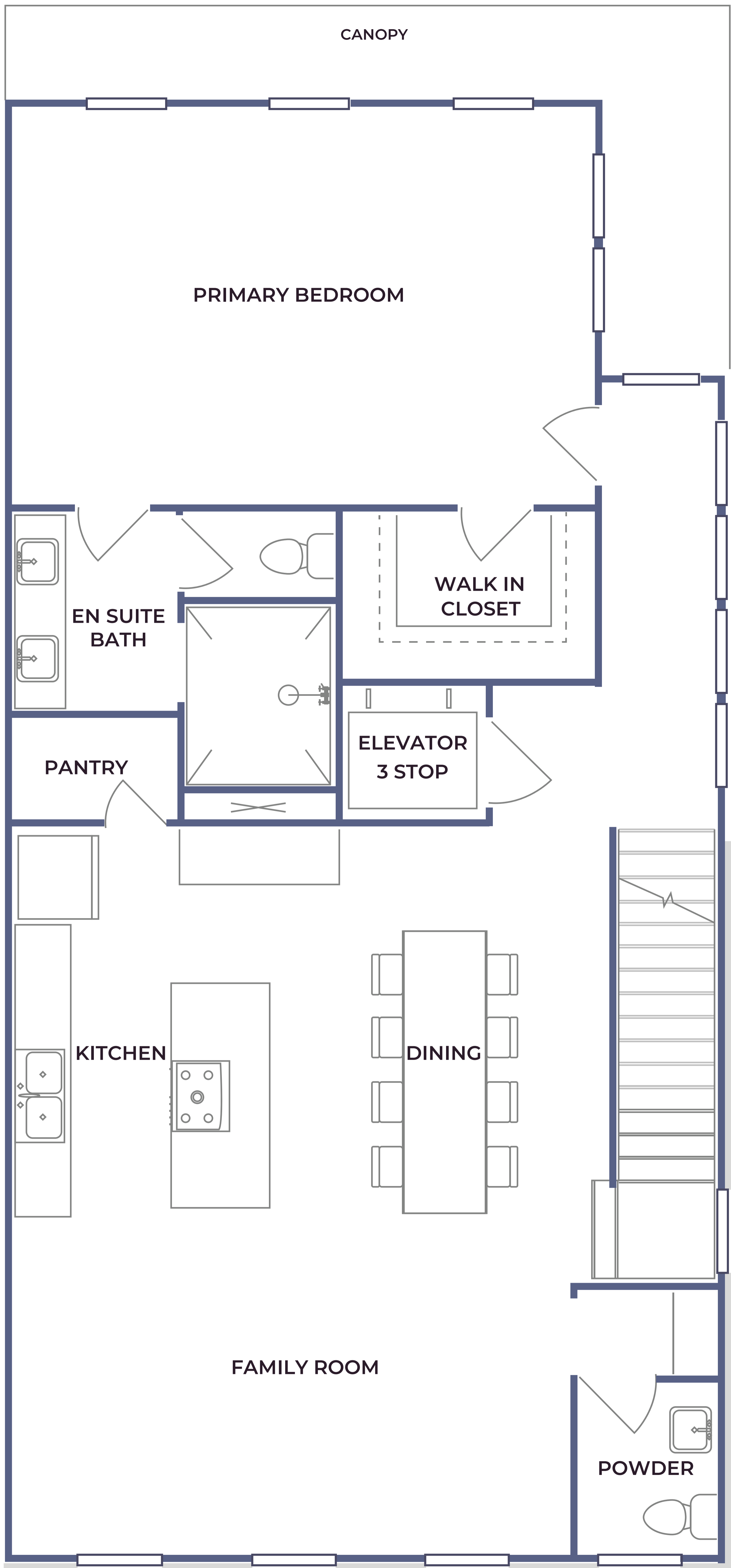
SECOND FLOOR PLAN Building 2, The Carlton end unit
