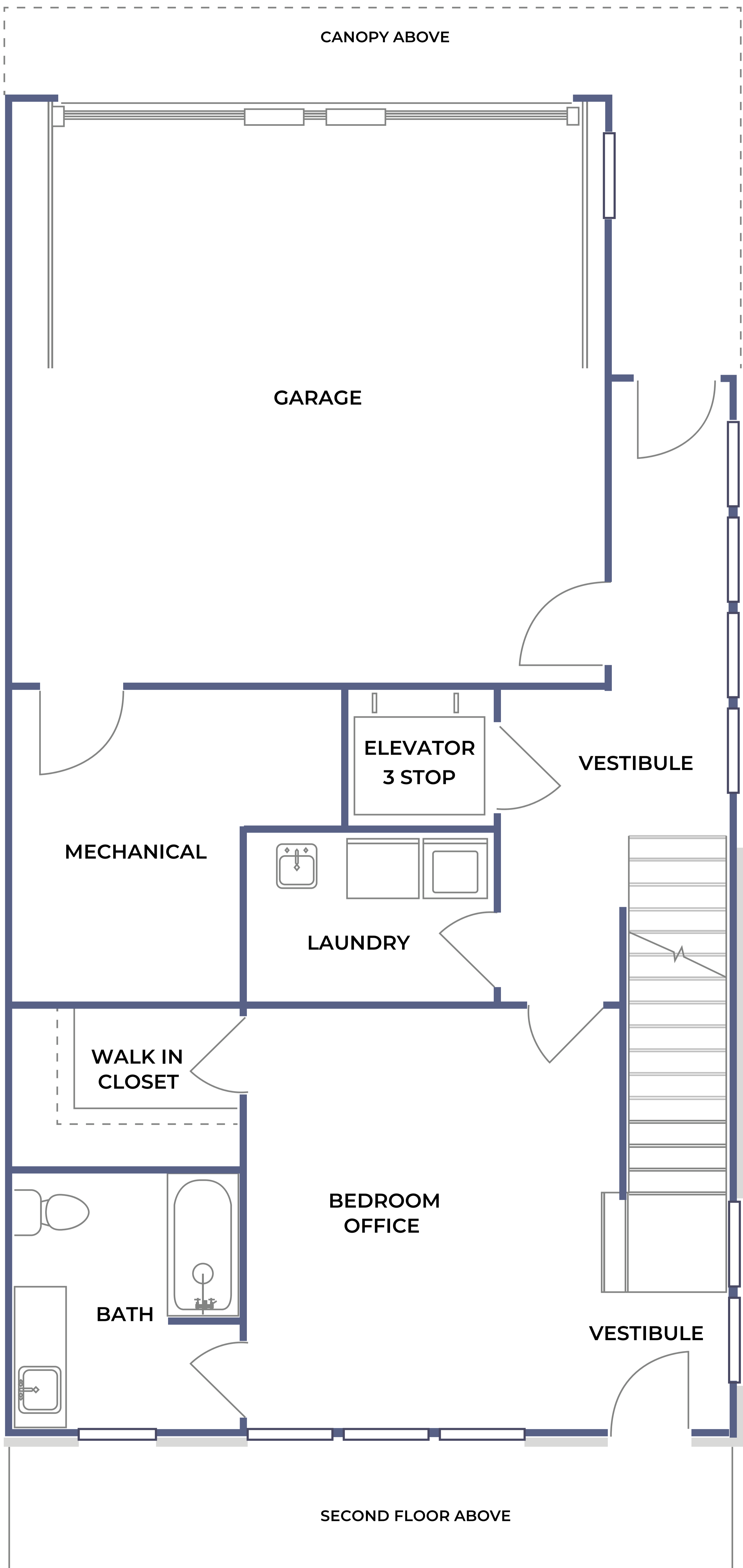
GROUND FLOOR PLAN Building 2, The Carlton end unit
