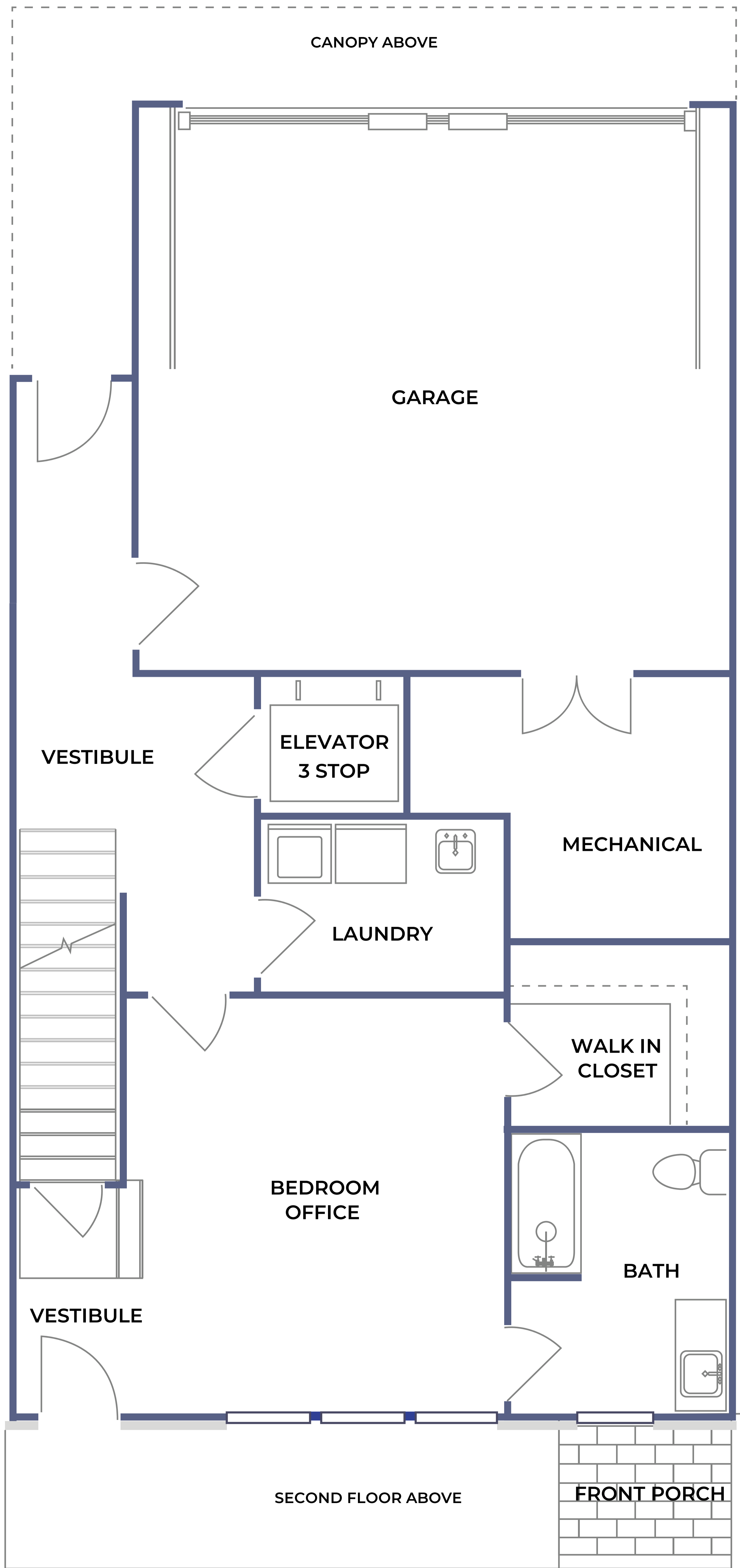
GROUND FLOOR PLAN Building 2, The Carlton interior unit
