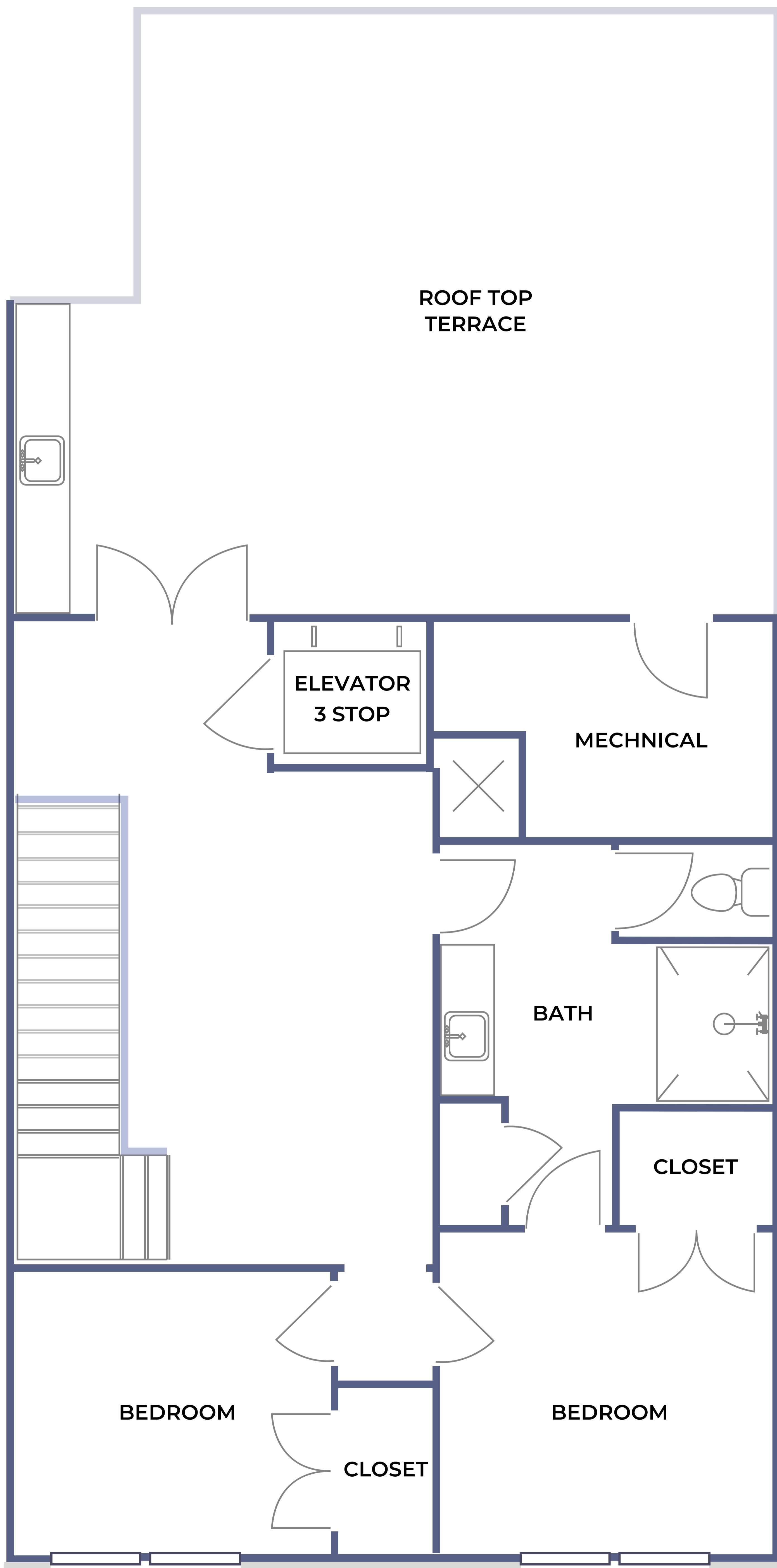
THIRD FLOOR PLAN Building 2, The Carlton interior unit
