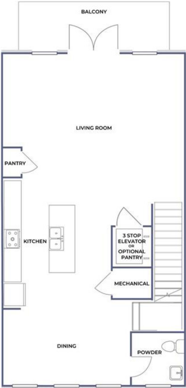
SECOND FLOOR PLAN The Adams interior unit *Optional elevator upgrade
